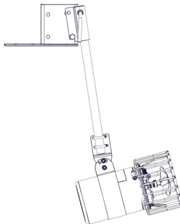
CUD unit with Universal Mount
