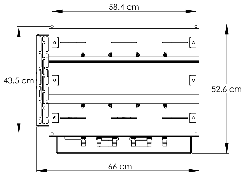
CABINET DIMENSIONS (cm)
